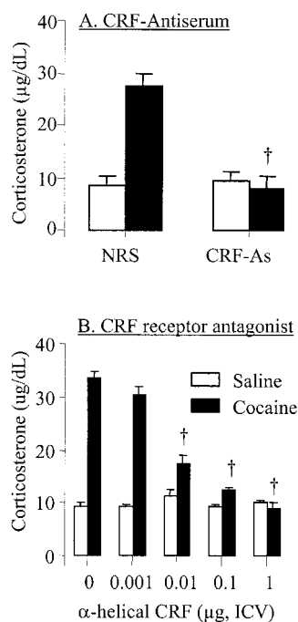
FIG. 1. Effects of a CRF antiserum and a CRF receptor antagonist (i.c.v.) on cocaine-induced corticosterone secretion in rats. A, pretreatment with a CRF-antiserum blocks ( \dagger p < 0.05 ) cocaine-induced increases in corticosterone levels. B, pretreatment with \alpha -helical CRF, a CRF receptor antagonist, attenuates ( \dagger p < 0.05 ) cocaine-induced increase in corticosterone levels. NRS, normal rabbit serum; CRF-As, CRF antiserum, 1:20 dilution. From Sarnyai Z (1998) Neurobiology of stress and cocaine addiction . Studies on corticotropin-releasing factor in rats, monkeys, and humans. Ann N Y Acad Sci 85:371–387 (Fig. 1). Data are presented with permission from The New York Academy of Sciences.
